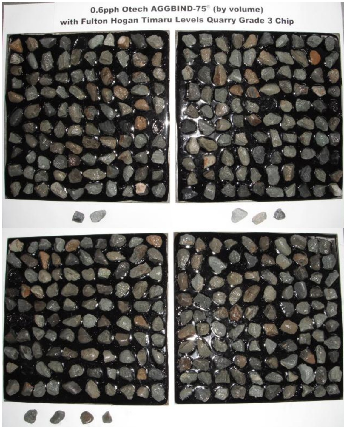
Figure 1. Photograph showing test plates with 180/200 bitumen and 0.6pph Otech AGGBIND-75® (by volume) after test was performed. Fulton Hogan Timaru - Levels Quarry grade 3 chip that was dislodged is arranged below the plates.
