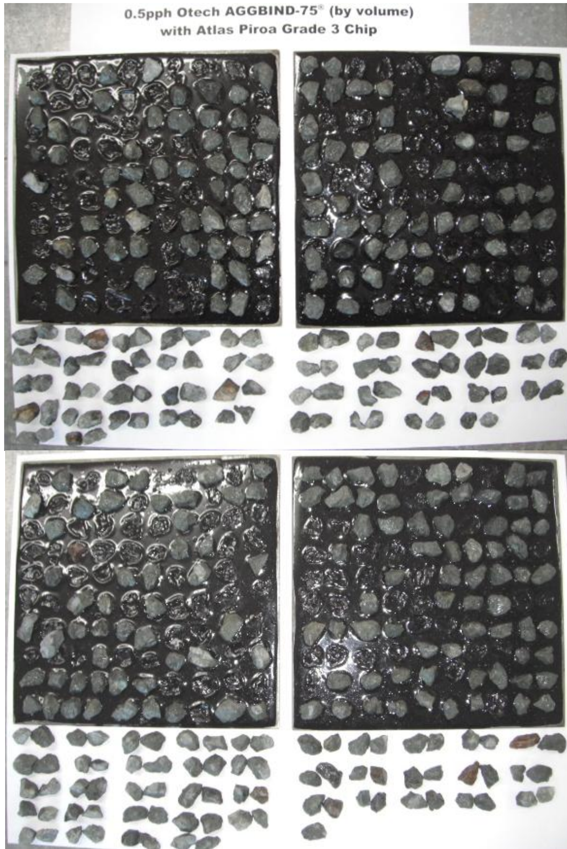
Figure 1. Photograph showing test plates with 180/200 bitumen and 0.5pph Otech AGGBIND-75® (by volume) after test was performed. Atlas Quarry – Piroa grade 3 chip that was dislodged is arranged below the plates.
