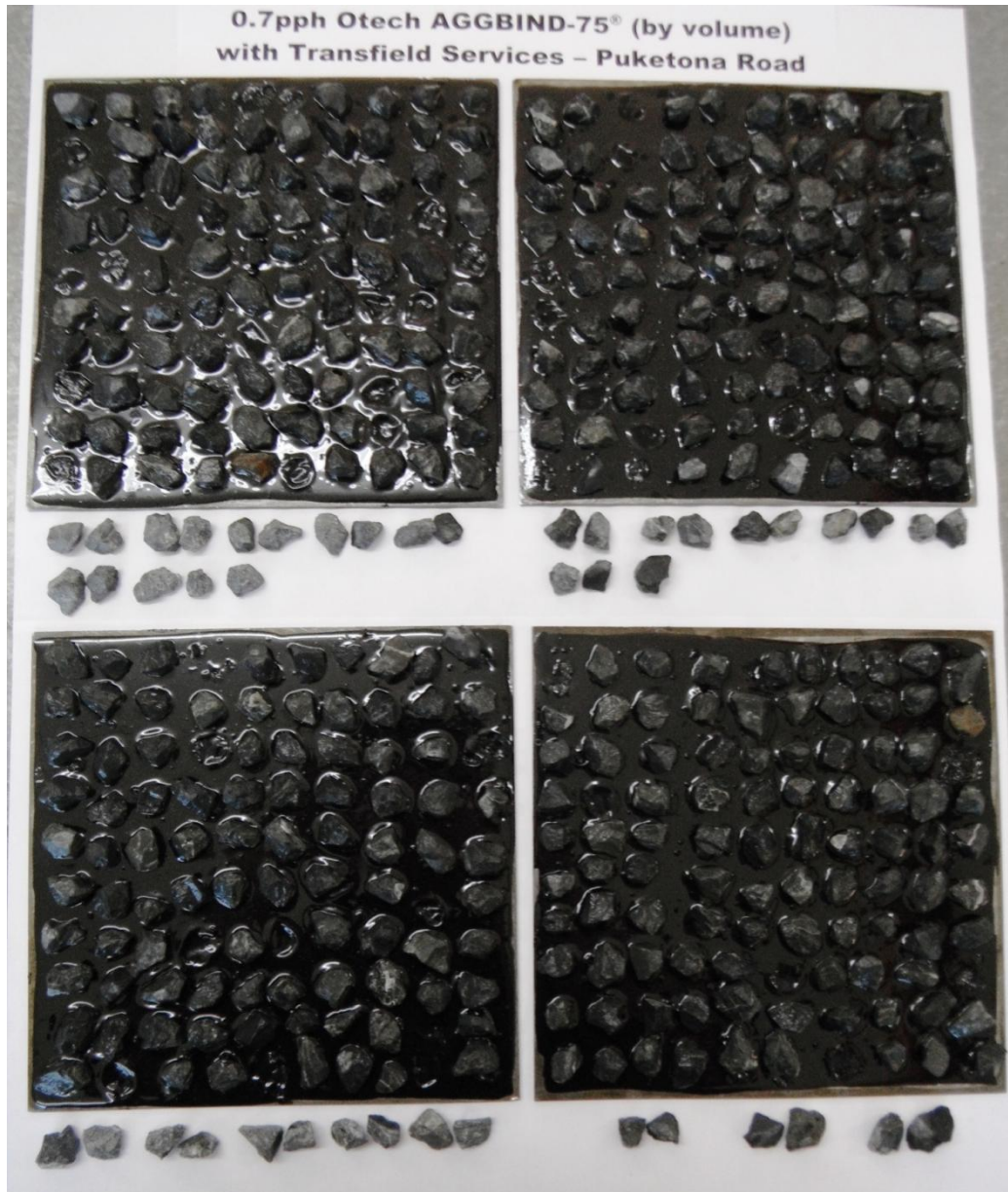
Figure 1. Photograph showing test plates with 180/200 bitumen and 0.7pph Otech AGGBIND-75® (by volume) after test was performed. Transfield Services – Puketona Rd grade 3 chip that was dislodged is arranged below the plates.
