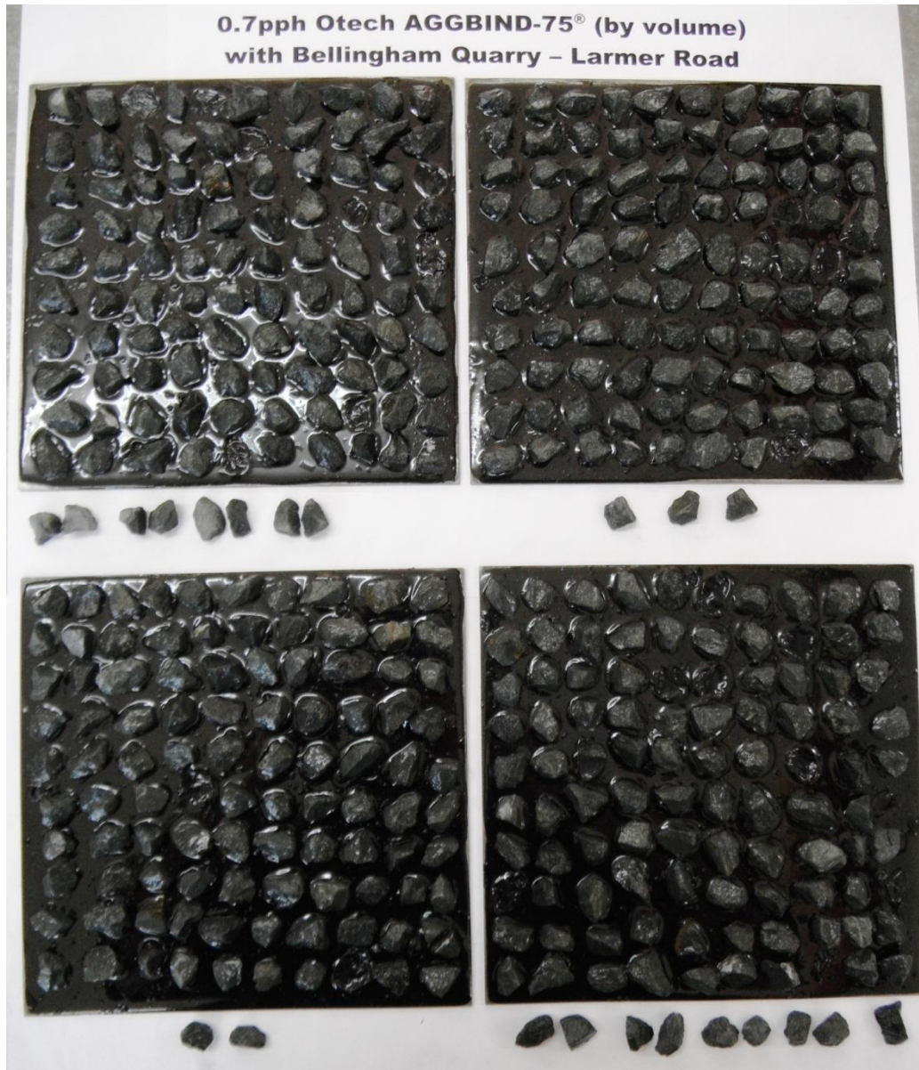
Figure 1. Photograph showing test plates with 180/200 bitumen and 0.7pph Otech AGGBIND-75® (by volume) after test was performed. Bellingham Quarry – Larmer Road grade 3 chip that was dislodged is arranged below the plates.
