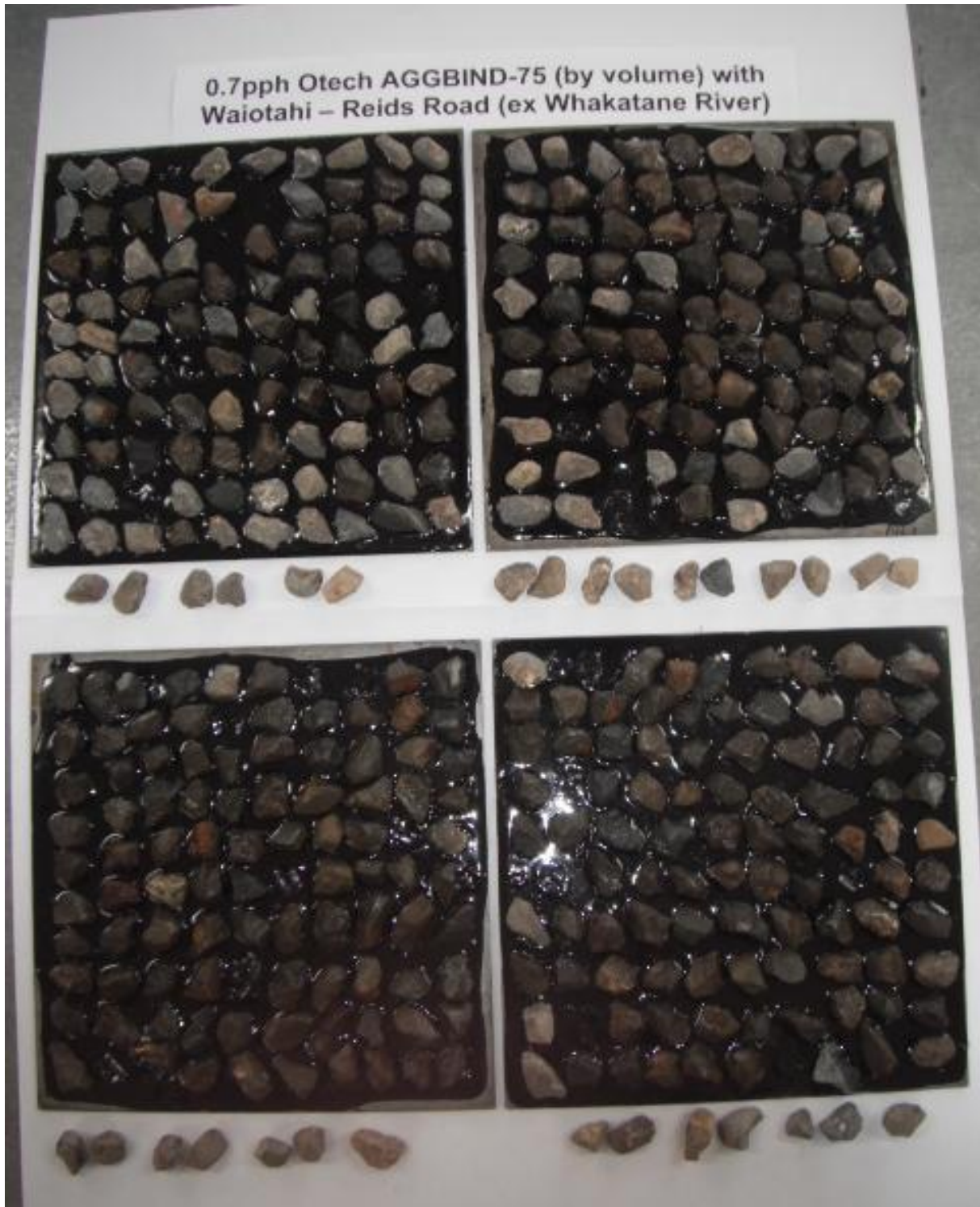
Figure 1. Photograph showing test plates with 180/200 bitumen and 0.7pph Otech AGGBIND-75 ® (by volume) after test was performed. Grade 3 Waiotahi – Reids Road chip that was dislodged is arranged below the plates.
