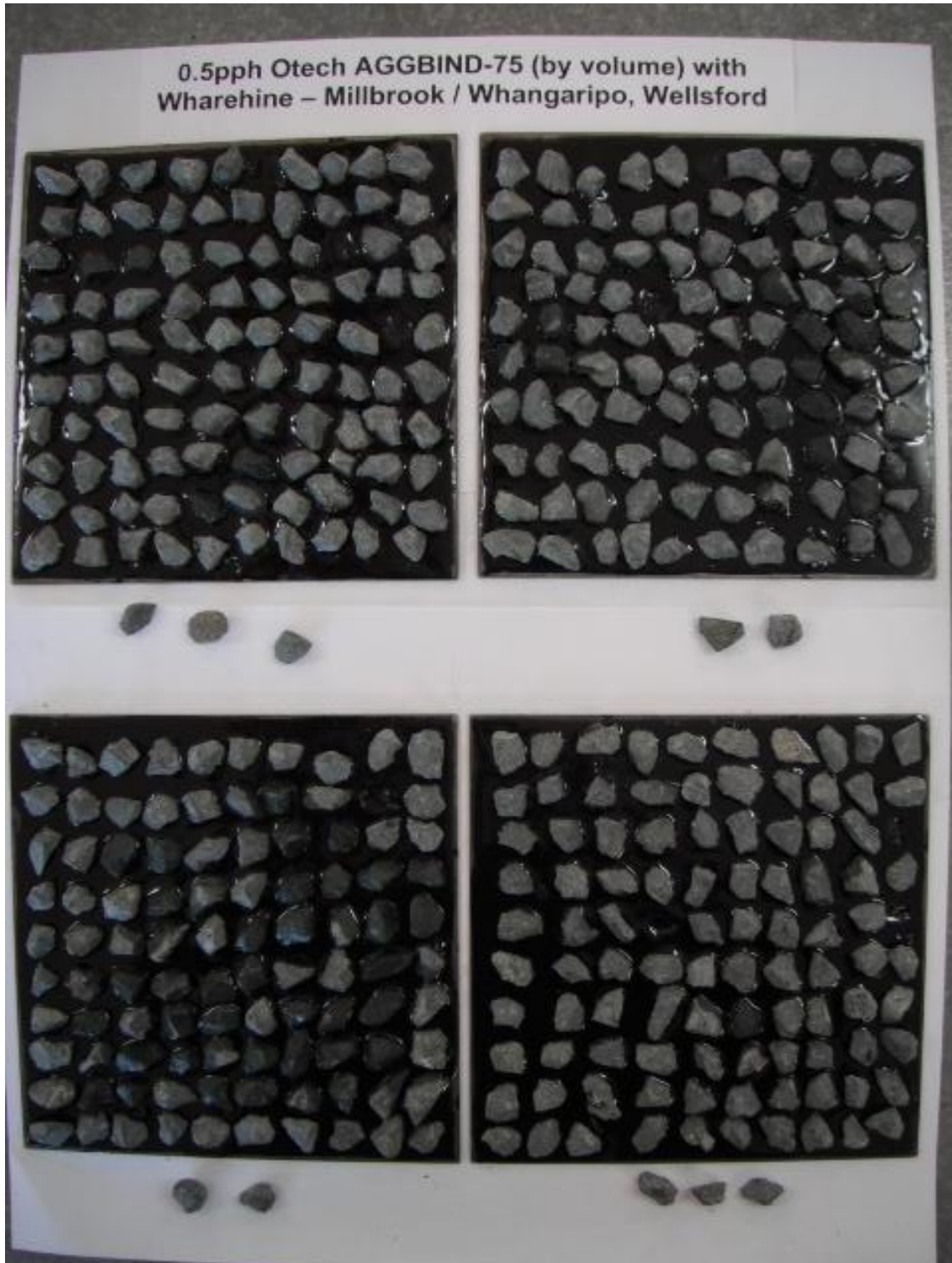
Figure 1. Photograph showing test plates with 180/200 bitumen and 0.5pph Otech AGGBIND-75® (by volume) after test was performed. Grade 3 Wharehine Millbrook Quarry / Whangaripo chip that was dislodged is arranged below the plates.
